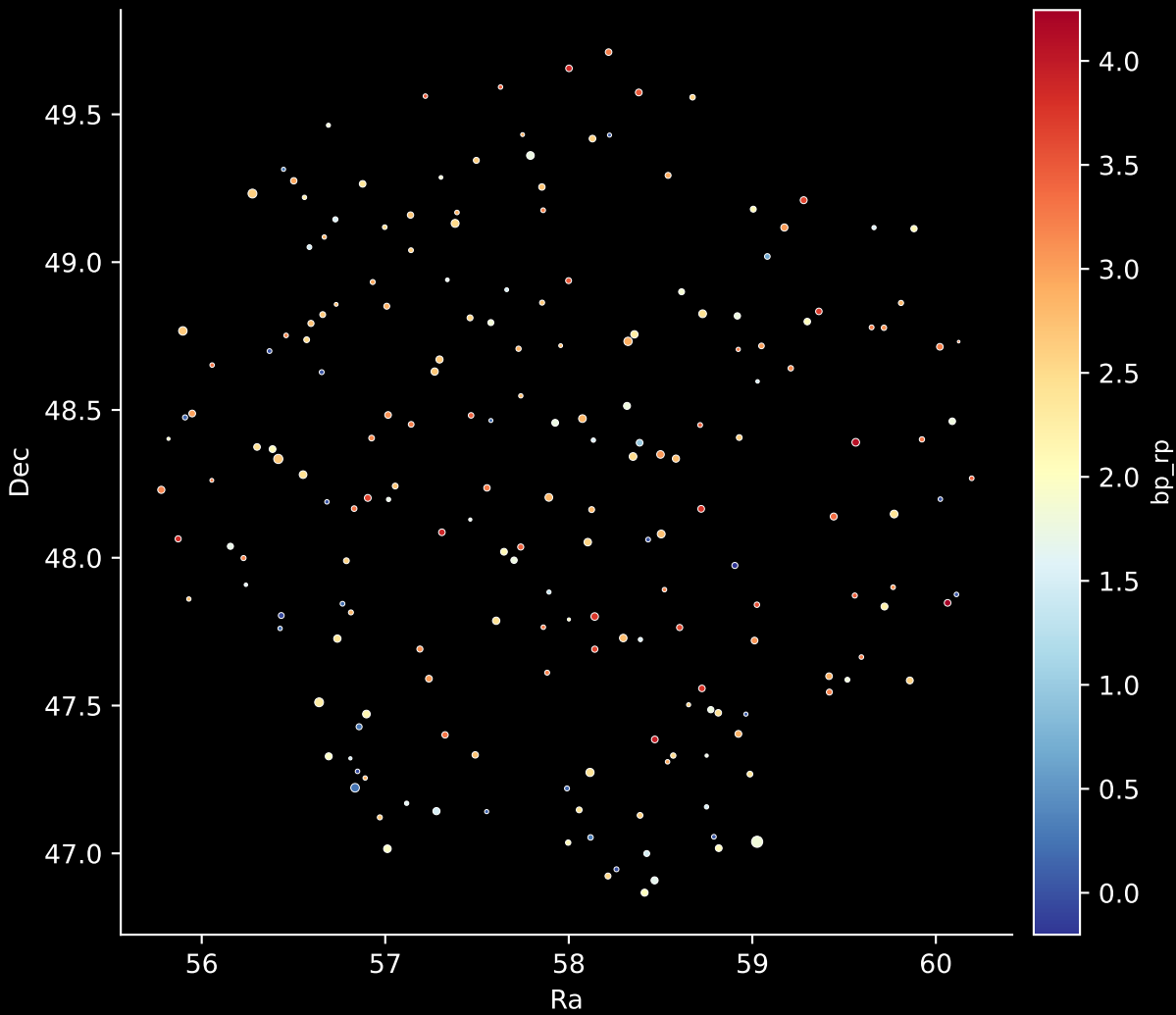
APOGEE DR17 Field: [090+00_btx] Stars: 199
