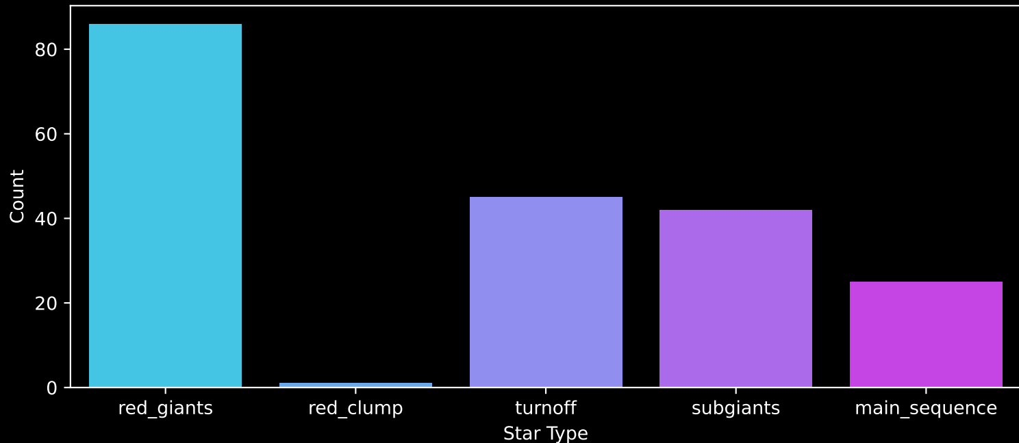
APOGEE DR17 Field: [090+00_btx] Count plot of Star Type
