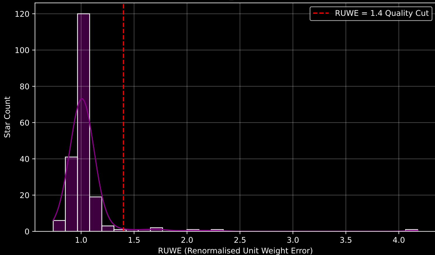
GAPOGEE DR17 Field [090+00_btx] RUWE Distribution (n= 197)
