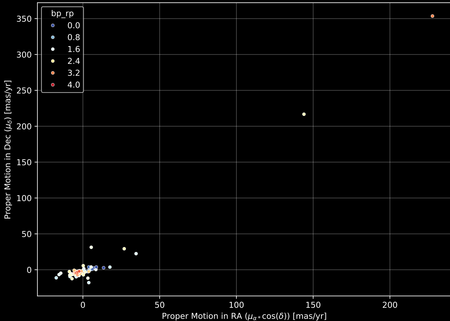
APOGEE DR17 Field: [090+00_btx] Proper Motion Diagram (n= 199)
