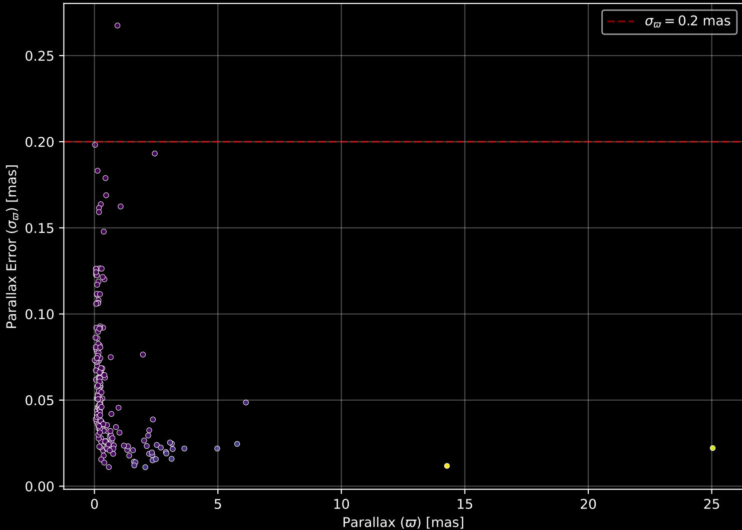
APOGEE DR17 Field: [090+00_btx] Parallax Quality (n= 199)
