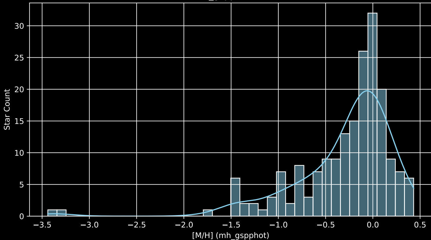
APOGEE DR17 Field: [090+00_btx [M/H] (mh_gspphot) (n= 190)
