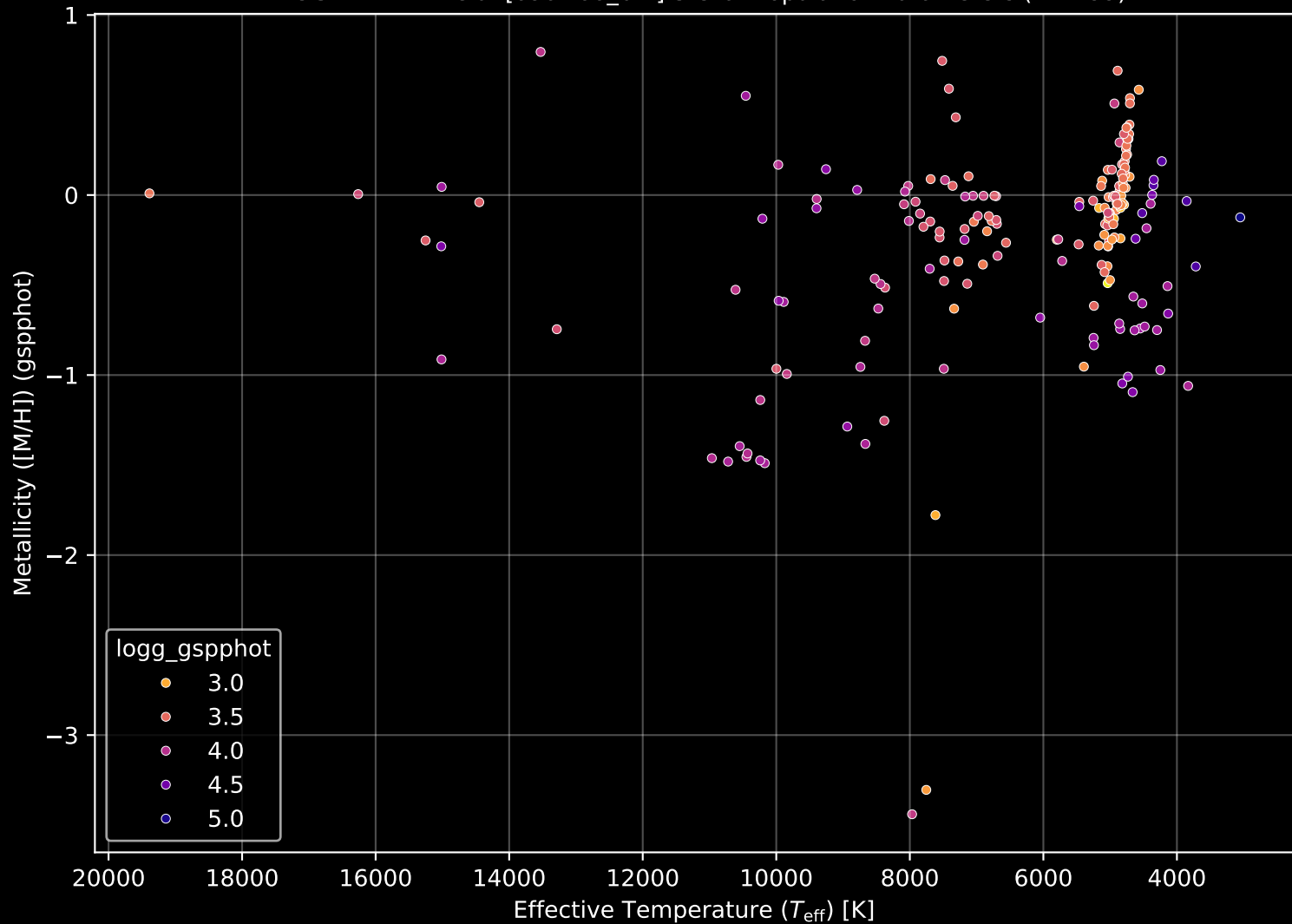
APOGEE DR17 Field: [090+00_btx] Stellar Population Parameters (n= 199)
